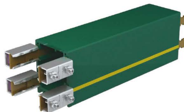
螺钉式接头安装示例 Bolted joints at powerail section
